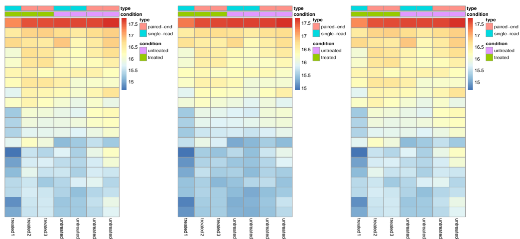
Figure 5: Heatmaps showing the expression data of the 20 most highly expressed genes. The data is of log2 normalized counts (left), from regularized log transformation (center) and from variance stabilizing transformation (right).
